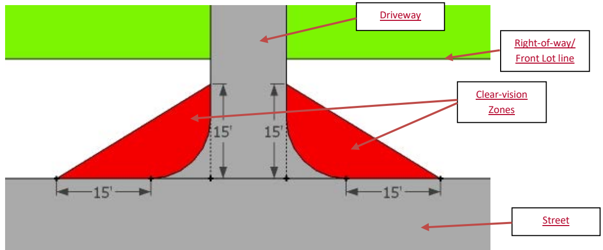
Figure 15.20(A): Residential Driveways
