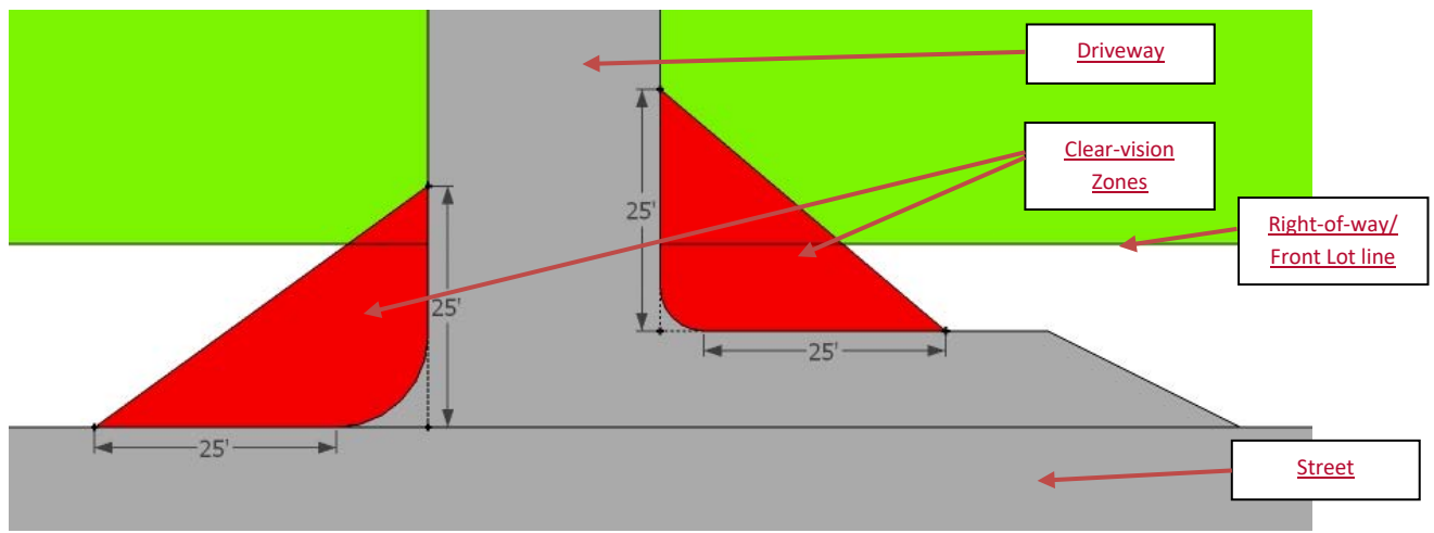
Figure 15.20(B): Commercial Driveways
