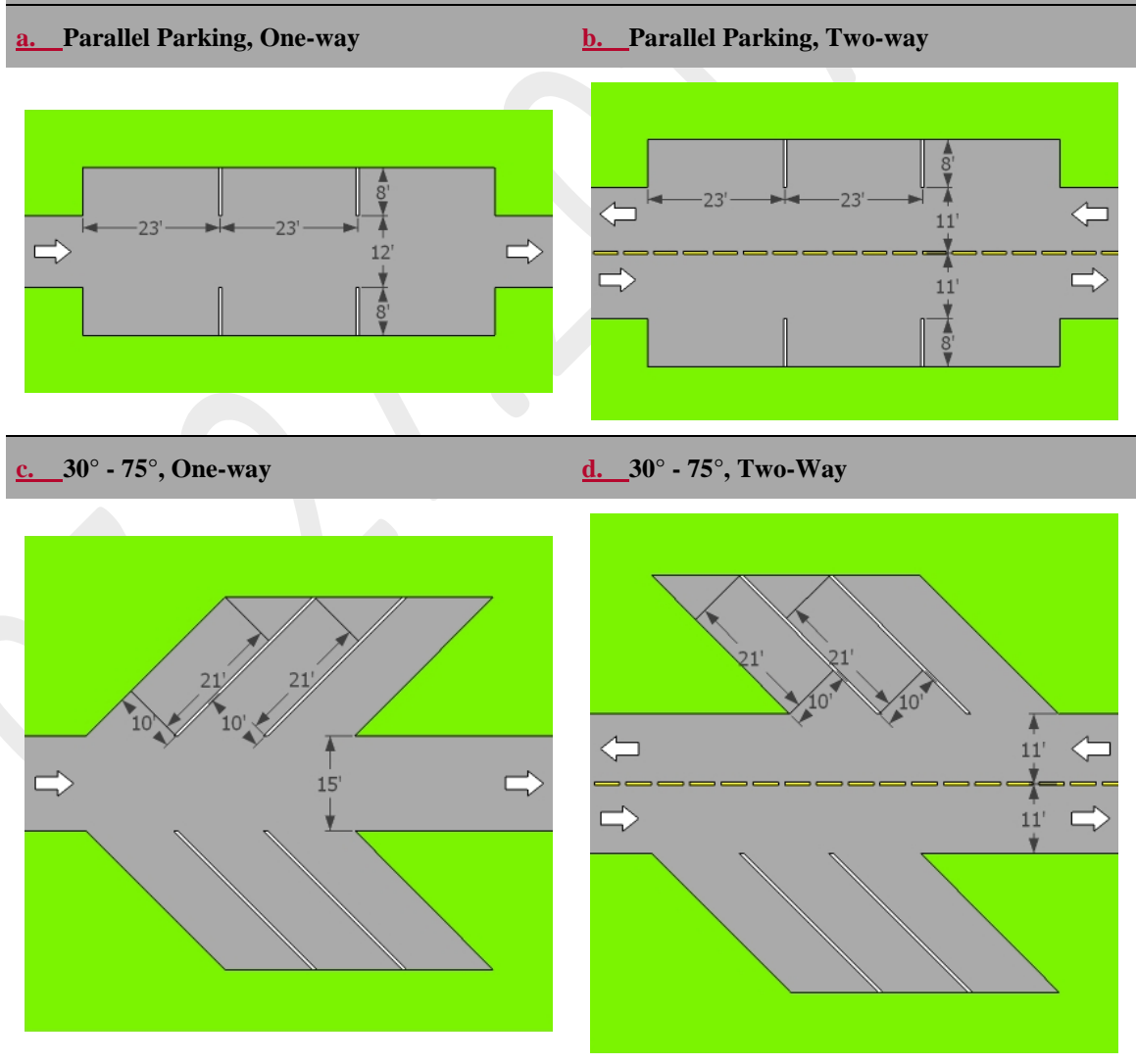
Figure 20.20(C)(7): Parking Space & Maneuvering Lane Configuration
